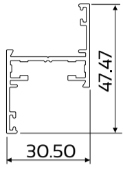
DIE No. W32027 Cas30.5 Frame 30mm Unequal Leg
