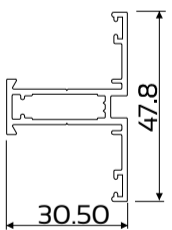
DIE No. W54867 Cas30.5 30mm Cottage Pane Mullion
