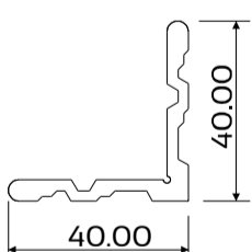
DIE No. W27989 Cas30.5 Corner Cleat 40mm
