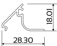
DIE No. W31139A Cas30.5 Bead Multi 13mm Gap
