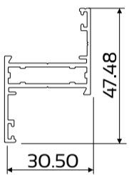
DIE No. W55684A Cas30.5 Sash Tubular
