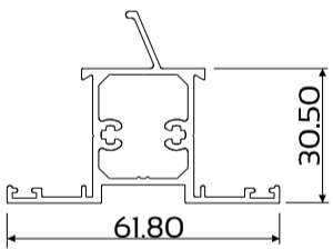
DIE No. W53630 Cas30.5 Mullion 30mm Weather Bar
