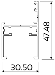
DIE No. W32028A Cas30.5 Frame 30mm Unequal Leg
