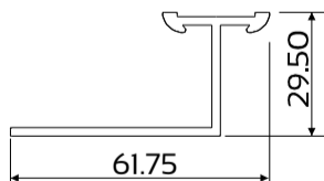
DIE No. W28002 Cas30.5 Fixing Lug Twist In
