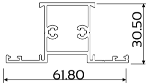
DIE No. W55685A Cas30.5 Mullion 30mm Standard
