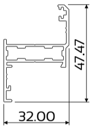
DIE No. W55441 Sash Picture Frame
