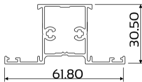
DIE No. W55008 Cas30.5 Mullion 30mm Econo
