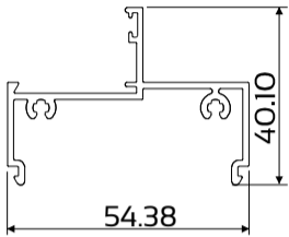
DIE No. W28481 Frame 54mm
