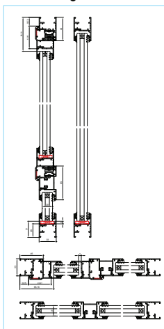
Typical sections Side Hung-D/G-EURO
